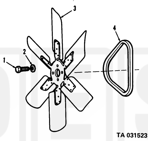
Figure 53A. Engine cooling fan and belt.
